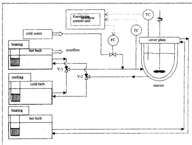
Figure 4. Reactor temperature control system for reactions with and without prepolymerization.
