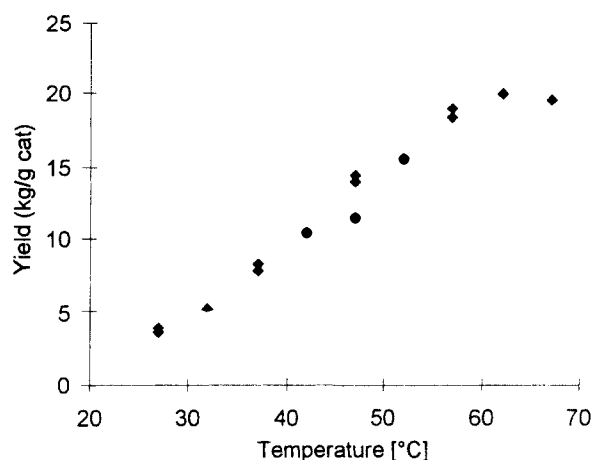
Figure 10. Polymer yield/g \text{MgCl}_2/\text{TiCl}_4/\text{EB} catalyst after 75-min reaction as a function of temperature.
