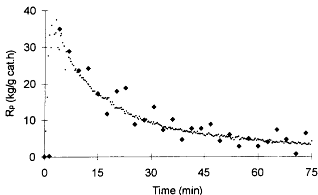
Figure 9. Reaction rate as a function of the time based on GC measurements (♦) and temperature difference over the reactor and the reactor jacket (●).
